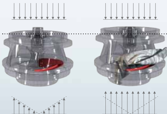
Fig 1: Hydraulic force distribution in normal operation
